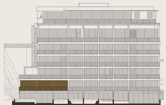
NORTH-WEST ELEVATION
