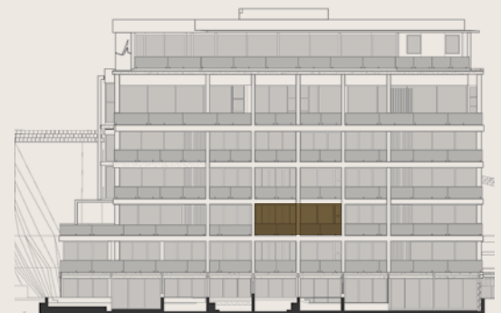
NORTH-WEST ELEVATION
